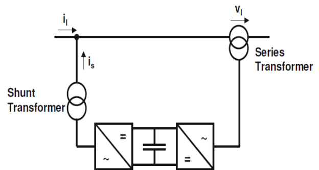
Fig 1. Principle Configuration of UPFC
