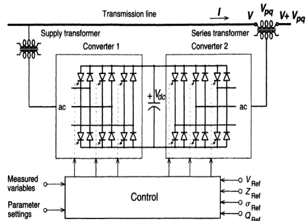
Fig 2. UPFC Control Structure
