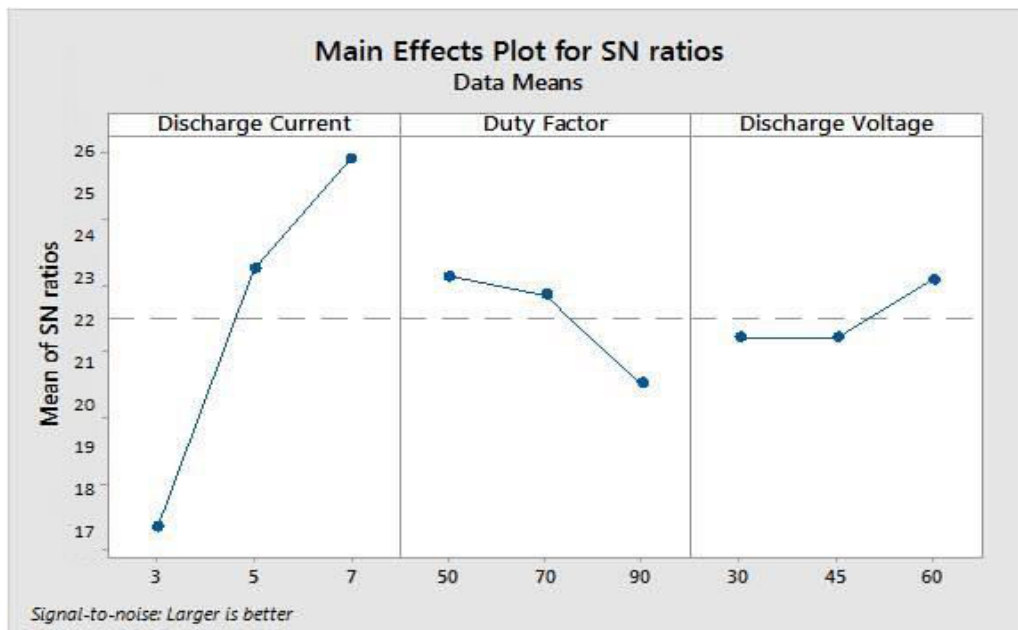
Fig. 3. S/N ratio graph for Material Removal Rate (MRR)
